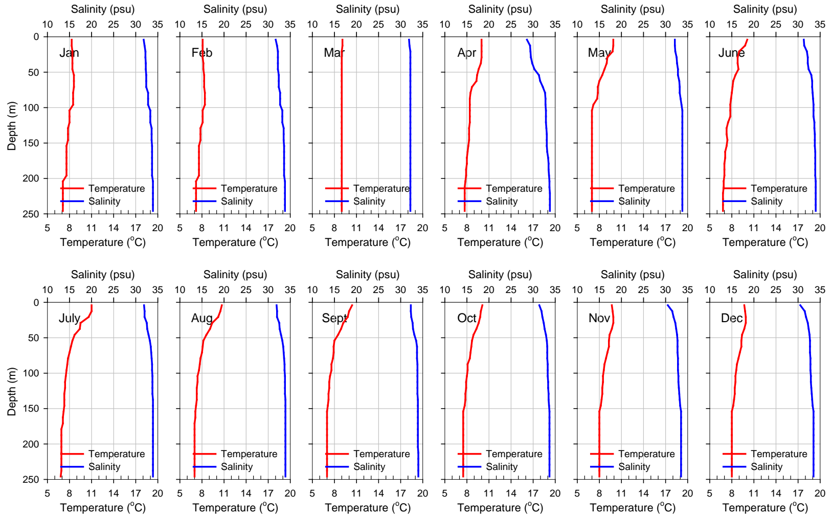
FIGURE 2-8 Temperature and Salinity Profiles at the Strait of Juan de Fuca Open Boundary
